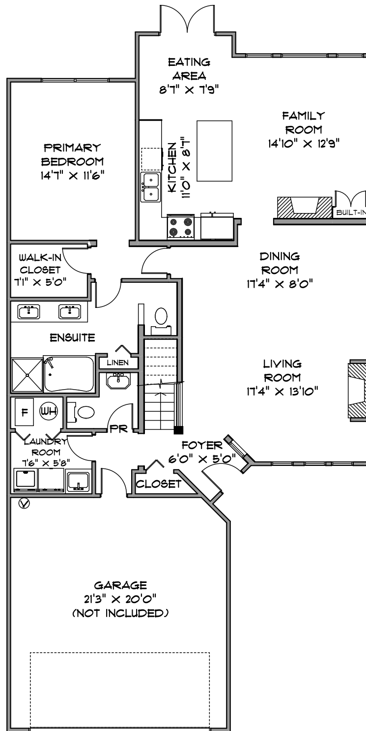
MAIN LEVEL 1337 SQ. FT.
